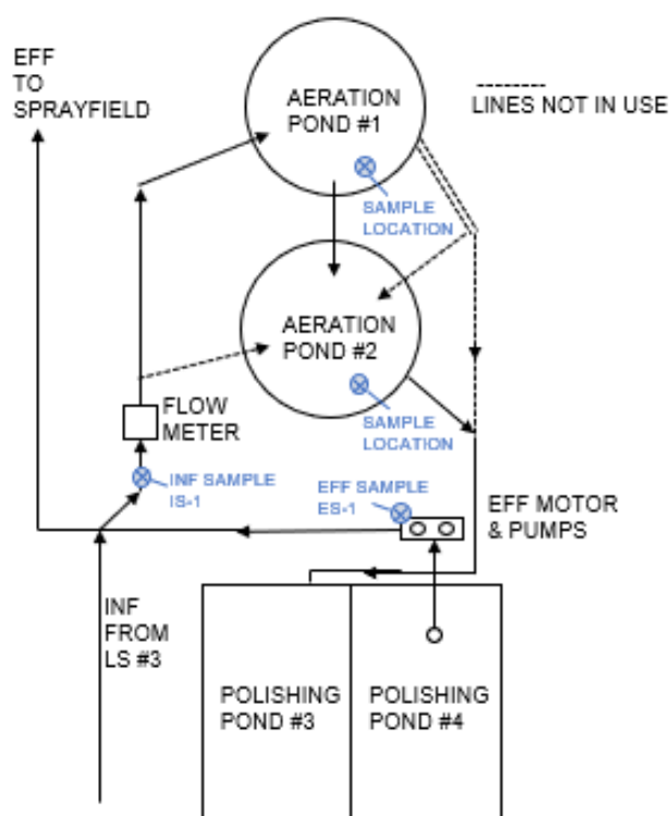
Figure 1. Process Flow Diagram with Sampling Locations. IS-1 and ES-1 represent compliance sampling locations. Sample locations at the aeration ponds are for process monitoring.
